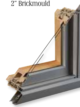
2" Brickmould
