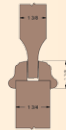
Raised Panel Molding W/ Standard Panel
