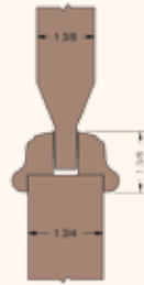
Raised Panel Molding W/ Traditional Panel
