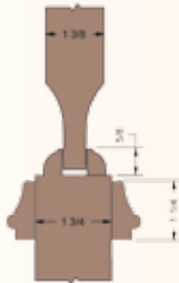
Recessed Molding W/ WB31 Bolection W/ Standard Panel
