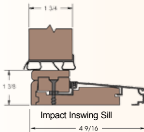
Available with 1 1/4", 2" or 3 1/4" exterior extensions
