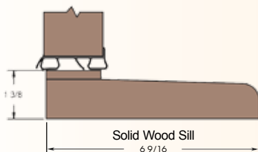
Available in a variety of depths.
