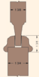
Raised Panel Molding W/ Classical Panel
