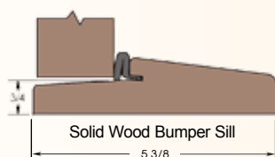
Available in a variety of depths.
