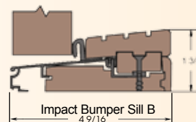
A 1 1/4" exterior extension is available for use with BMC
